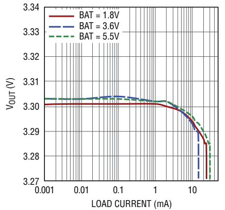
Buck-Boost Load Regulation, V_{OUT} = 3.3\text{V} , 100mA I_{PEAK} Setting
